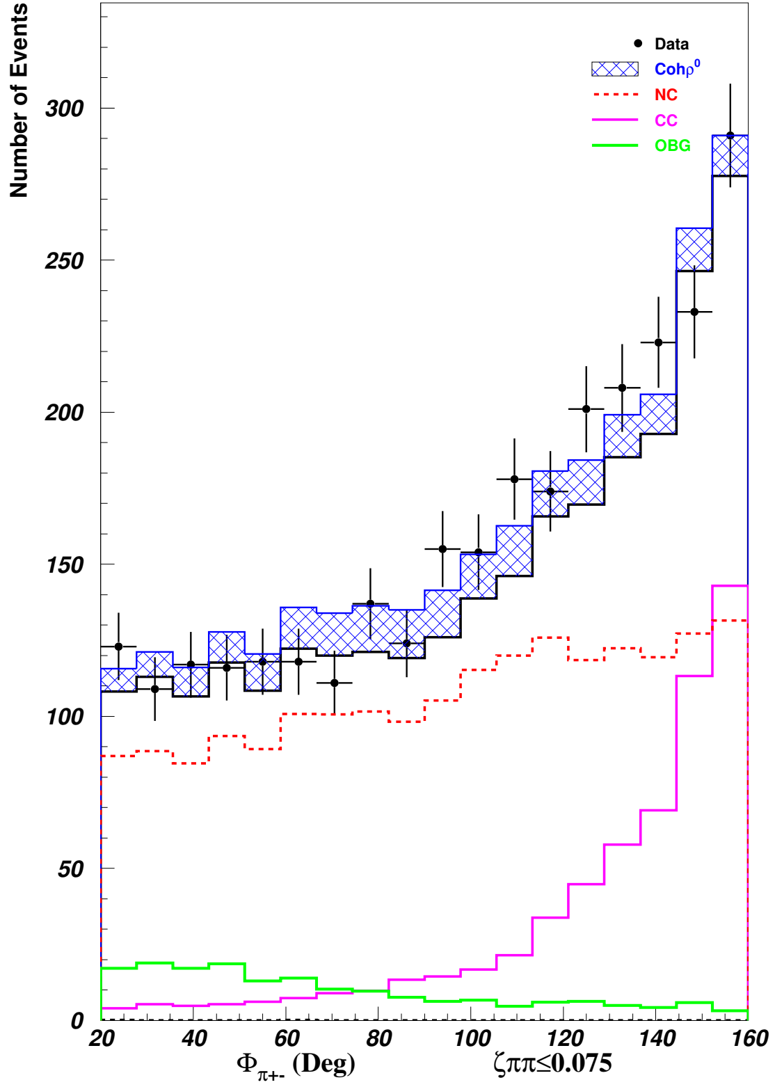
Figure 35: \phi_{12} (Signal Region)
