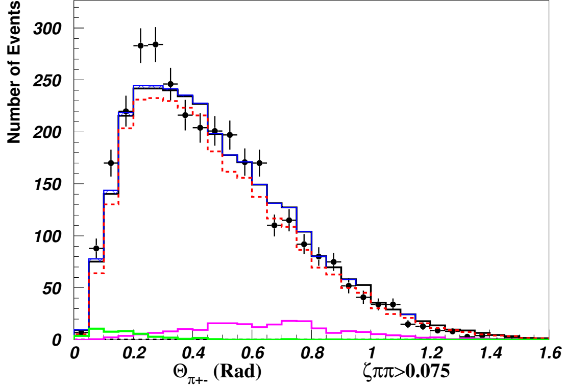
Figure 45: \theta_{\pi\pi} and \theta_{12} (Background Region)
