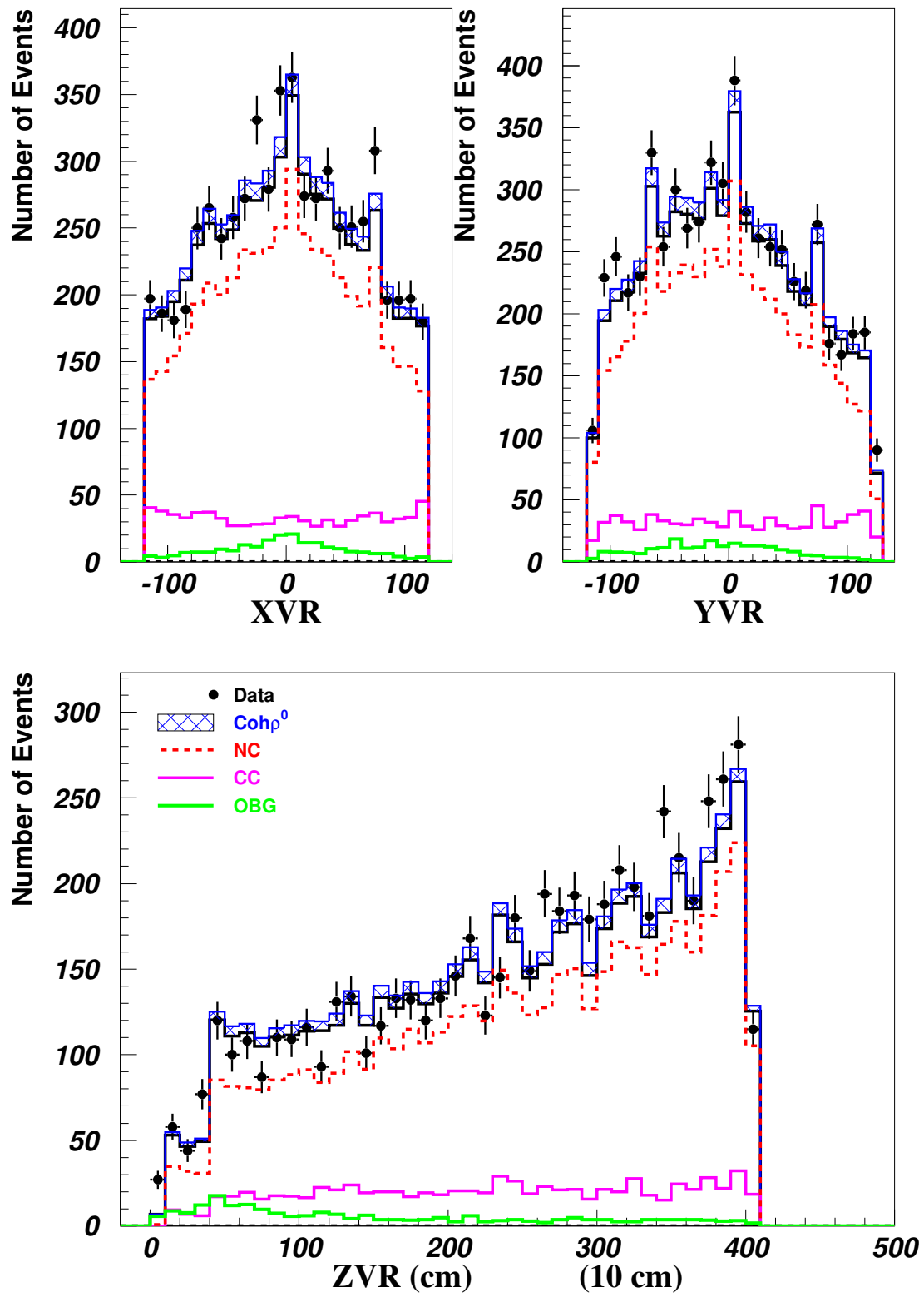
Figure 17: Vertex Position
