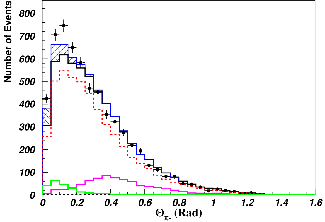
Figure 40: \theta_{\pi^+} and \theta_{\pi^-}
