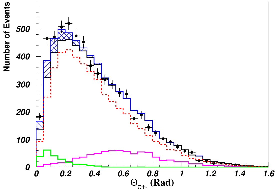
Figure 43: \theta_{\pi\pi}
