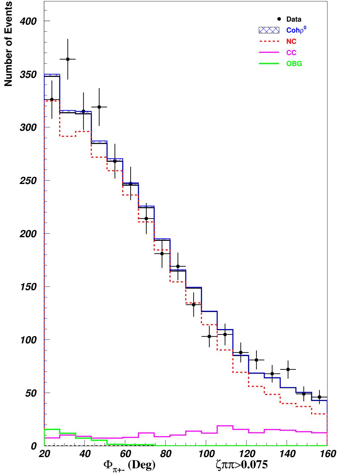
Figure 36: \phi_{12} (Background Region)
