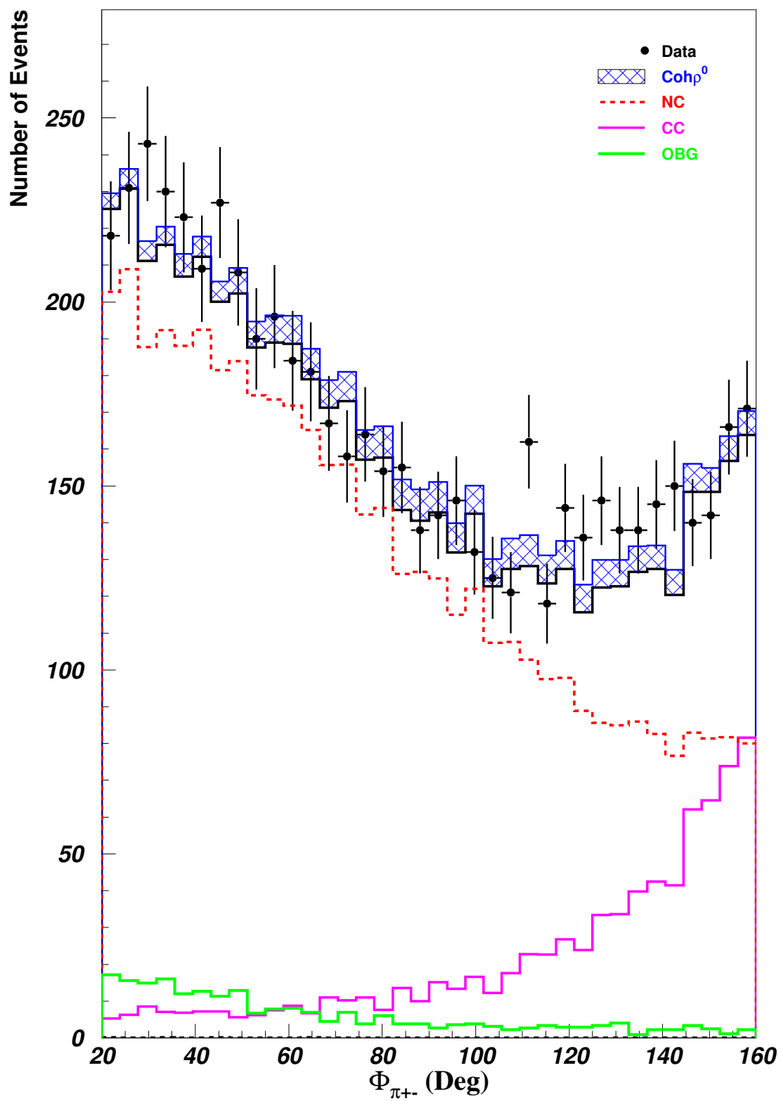
Figure 31: \phi_{12}
