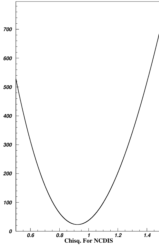
Figure 1: 1\sigma \chi^2 plot for NCDIS
