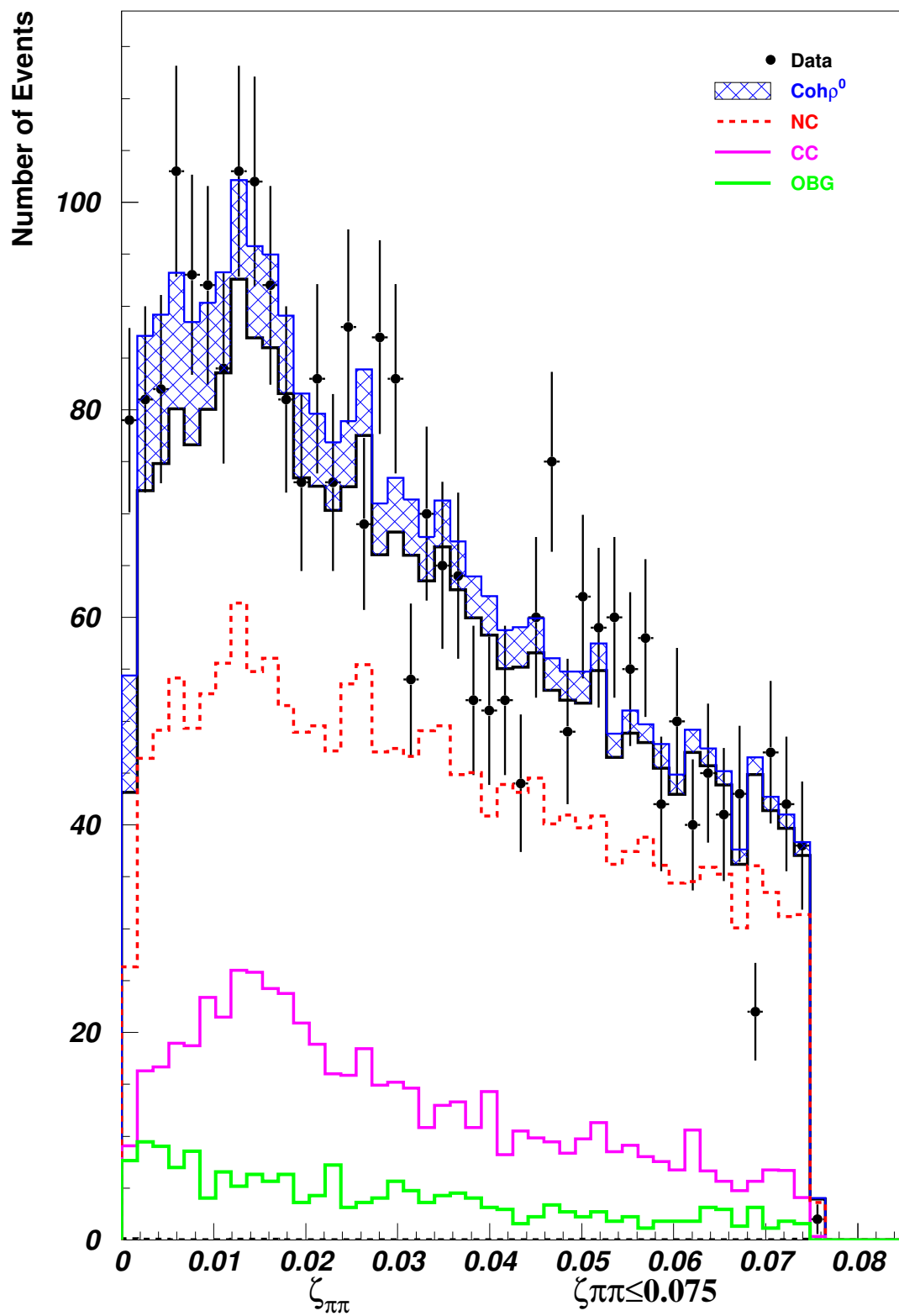
Figure 26: \zeta_{\pi\pi} (Signal Region)
