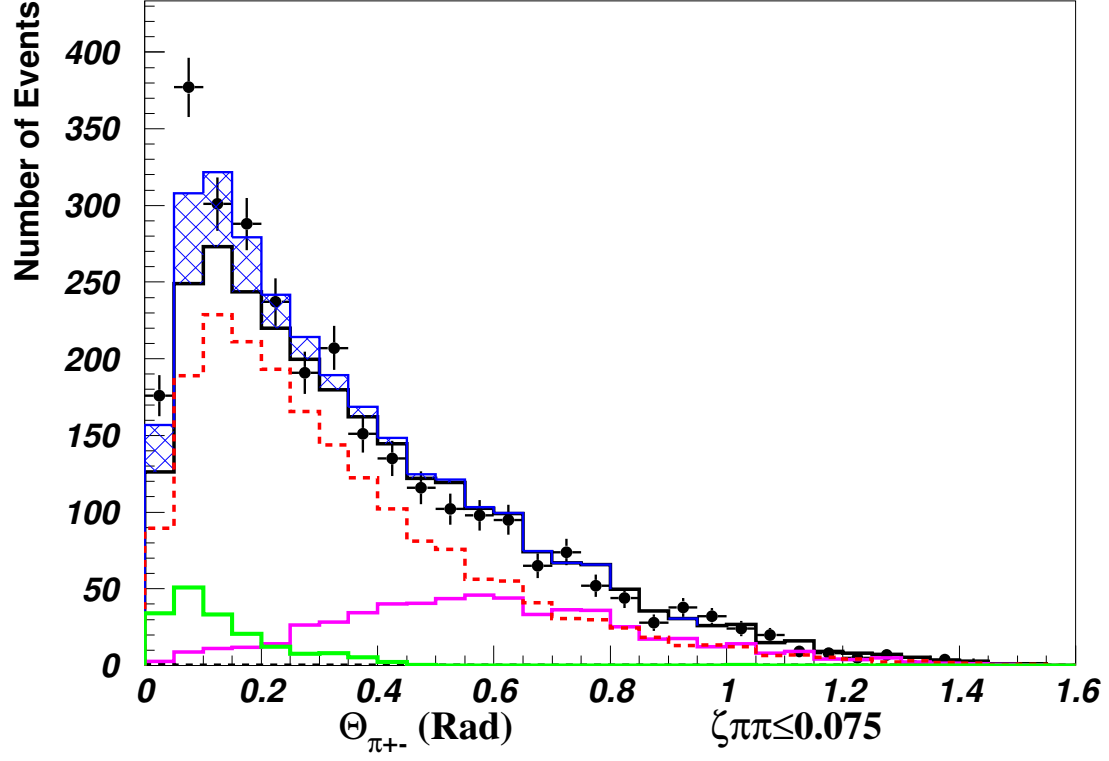
Figure 44: \theta_{\pi\pi} and \theta_{12} (Signal Region)
