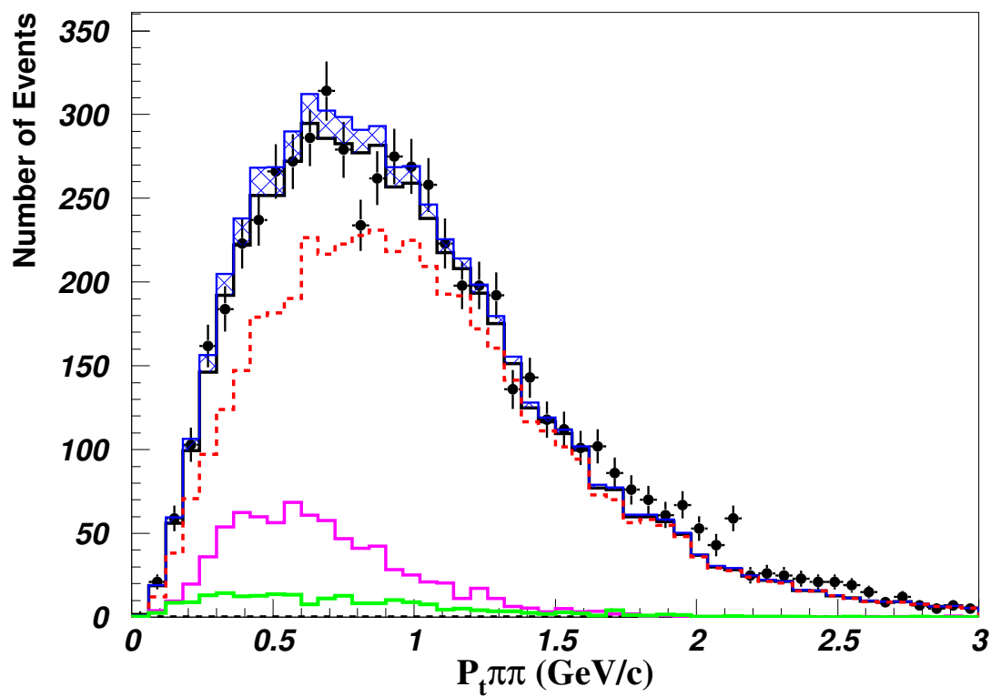
Figure 50: P_t \pi\pi
