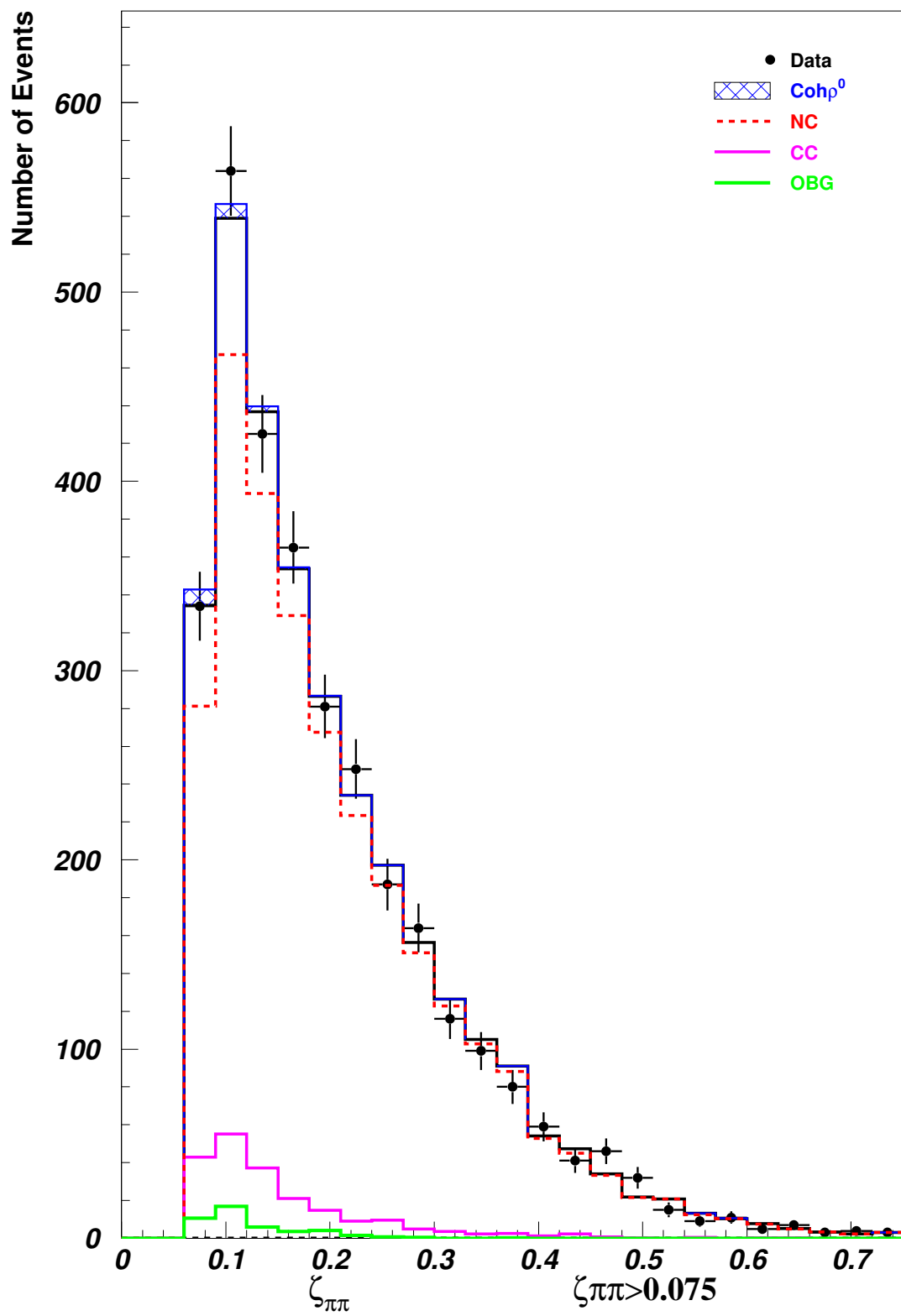
Figure 27: \zeta_{\pi\pi} (Background Region)
