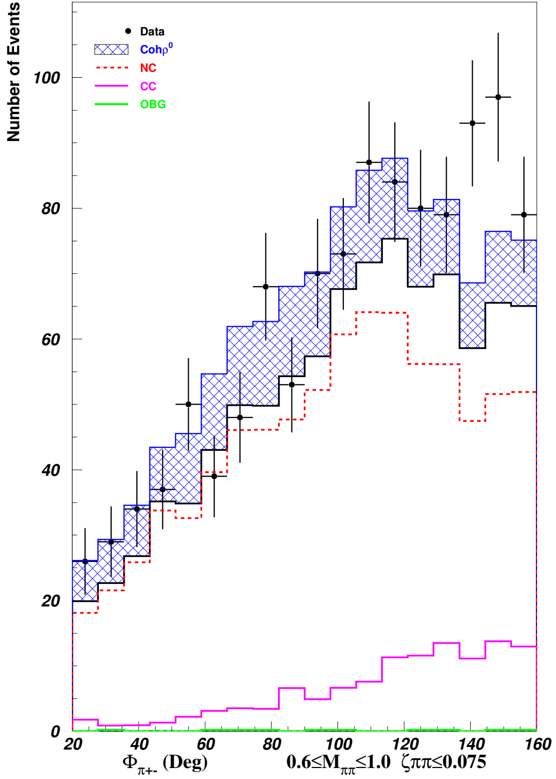
Figure 33: \phi_{12} (Signal Region in Rho Mass)
