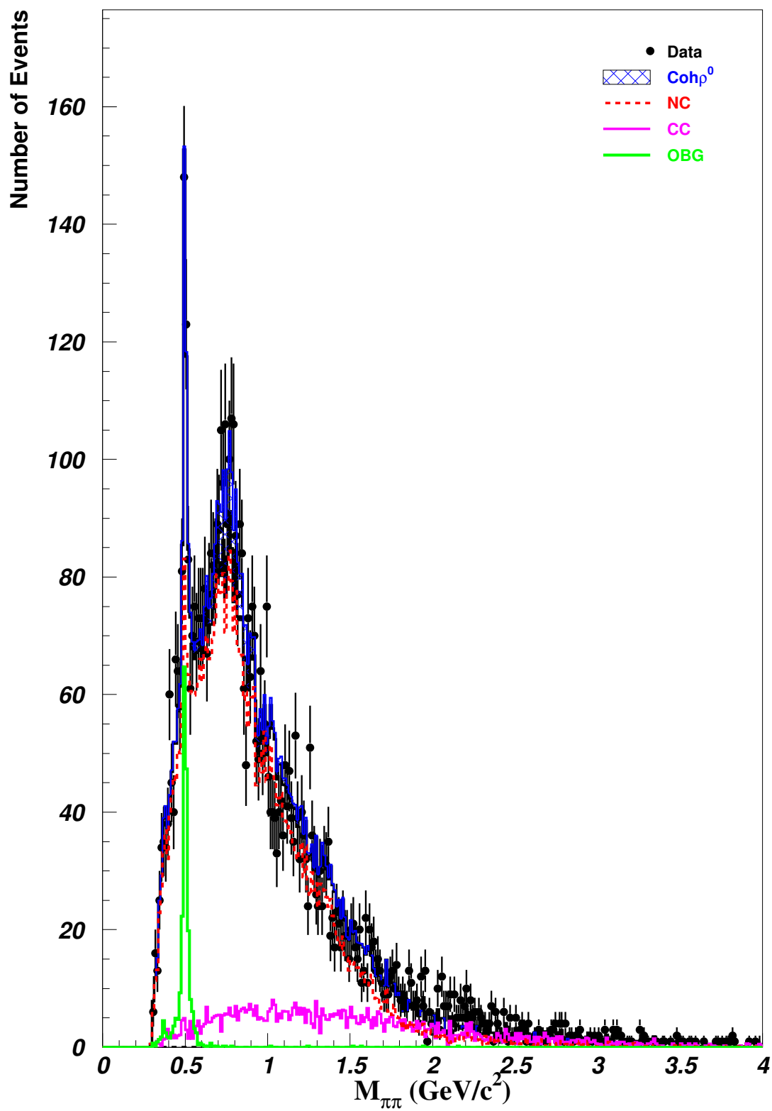
Figure 18: M_{\pi\pi} 12.5MeV
