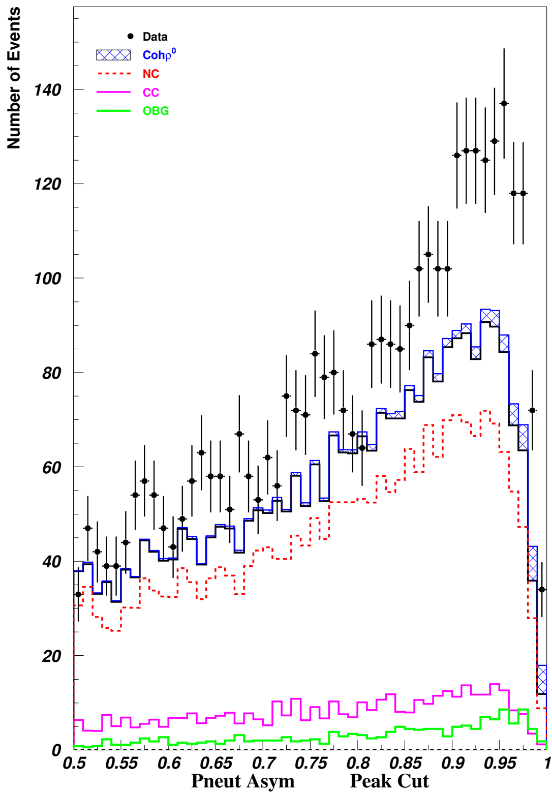
Figure 62: PAN (Neutral Momentum Asymetry)
