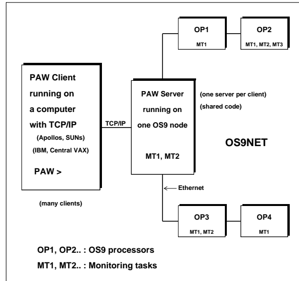
Figure 9.3: Visualising histograms on OS9 modules from PAW
