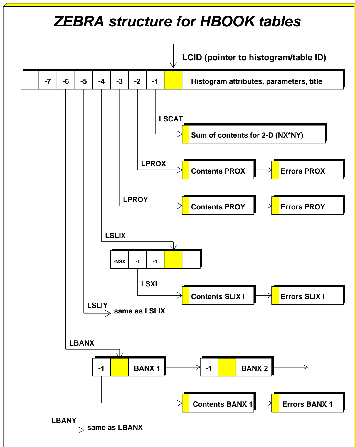
Figure 8.2: The zebra data structure used for two-dimensional histograms
